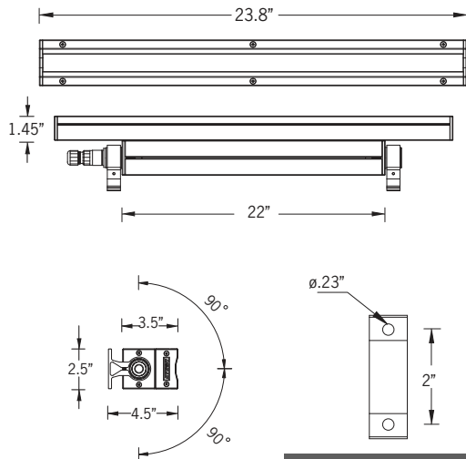
Mounting Detail
